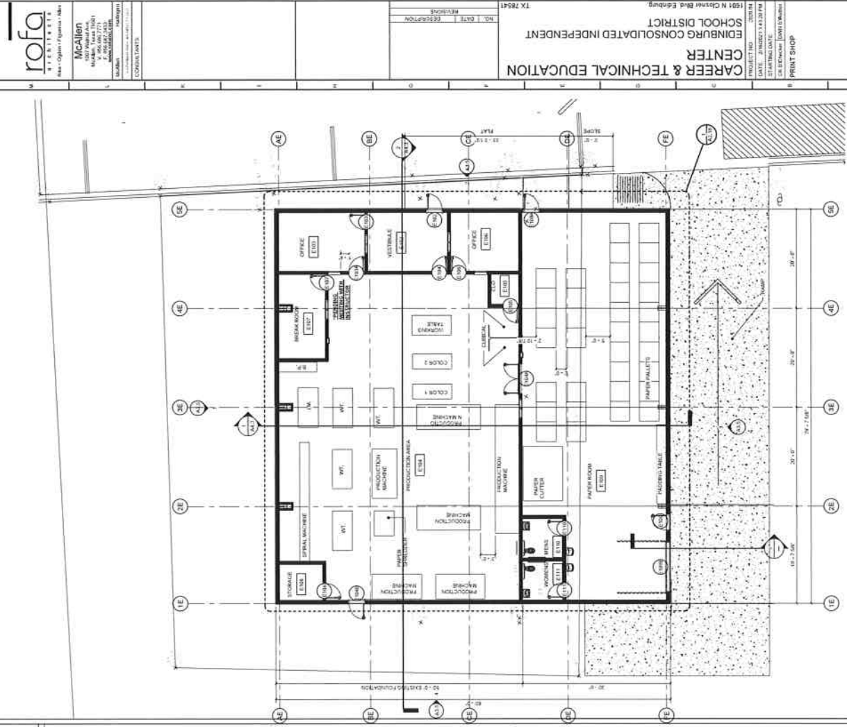
PROPOSED PRINT SHOP
